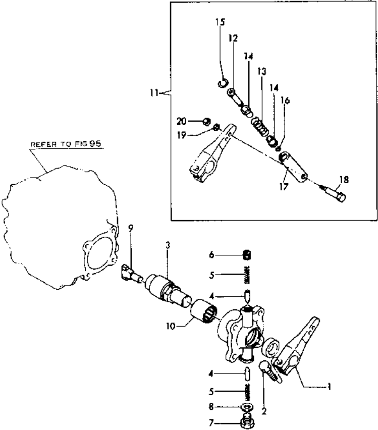
Fig.98 操縦装置 REMOTE CONTORL DEVICE
