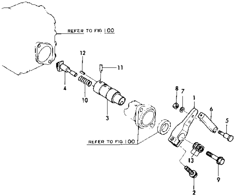
Fig.103 操縱裝置 REMOTE CONTOROL DEVICE
