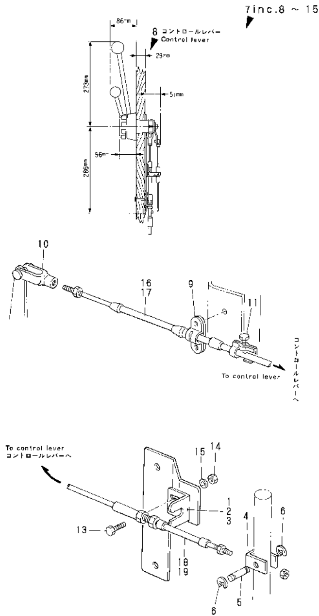
Fig.16. REMOTE-CONTROL DEVICE(OPTIONAL)
