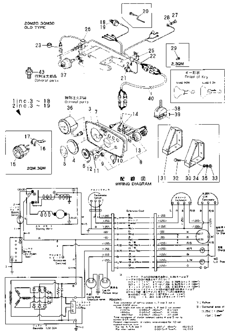
Fig.20. INSTRUMENT PANEL
