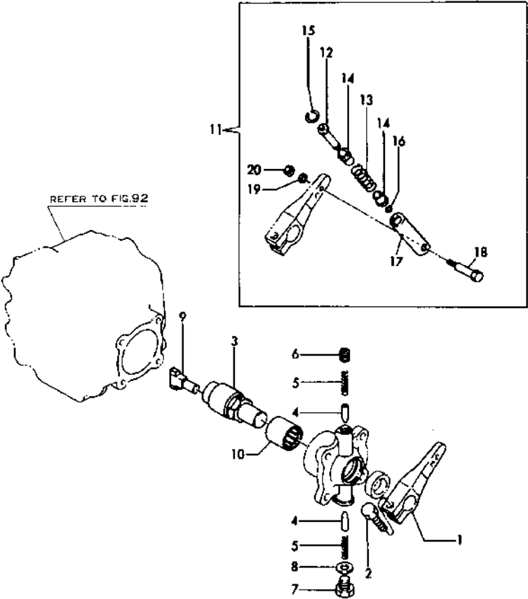
Fig. 95 操纵装置 REMOTE CONTORL DEVICE
