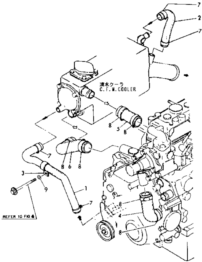
Fig.39 冷却水パイプ(淡水) COOLING FRESH WATER PIPE
