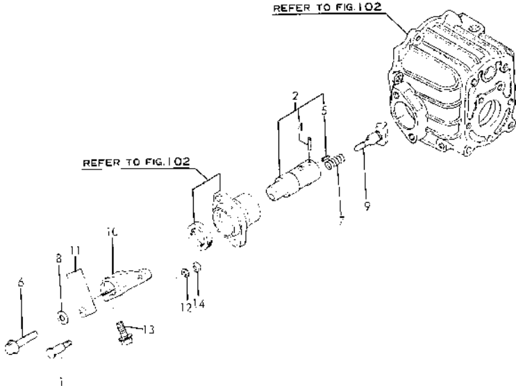
Fig.109 操縱装置 REMOTE CONTOROL DEVICE
