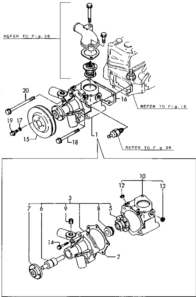
Fig.32. COOLING FRESH WATER PUMP
