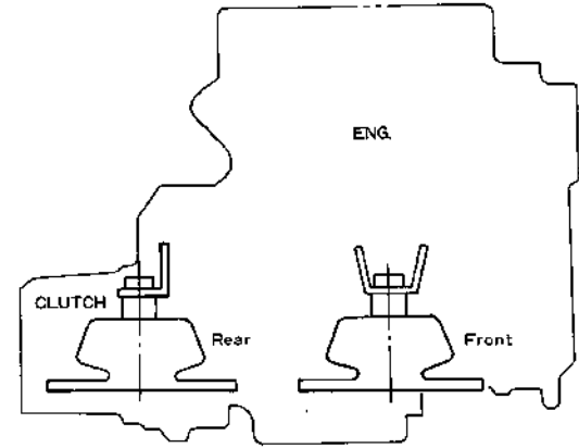
Fig.56. FLEXIBLE MOUNTING(OPTIONAL)
