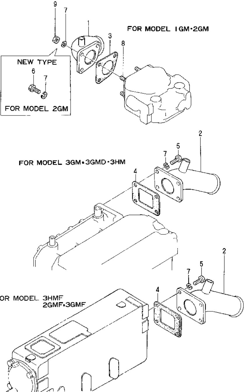
Fig.15. MIXING ELBOW
