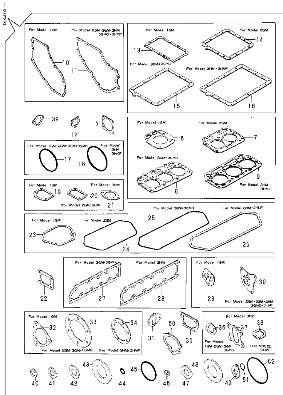
Fig.65. GASKET KIT(OPTIONAL)
