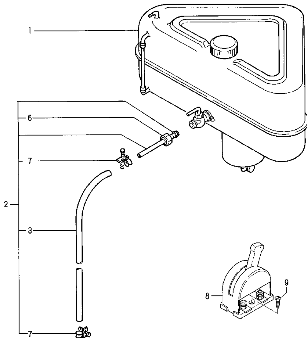
Fig.58. FUEL OIL TANK & BATTERY SWITCH(OPTIONAL)
