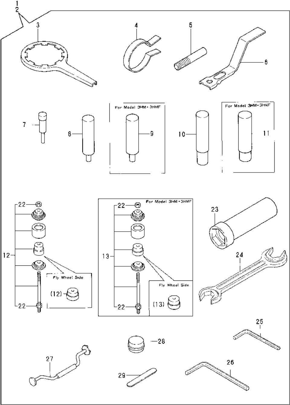
Fig.63. SPECIAL TOOL(OPTIONAL)
