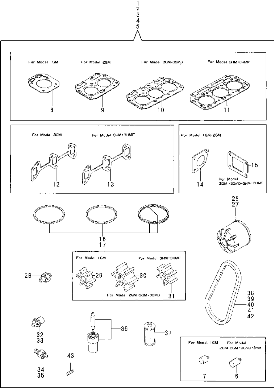
Fig.64. REPAIR KIT(OPTIONAL)
