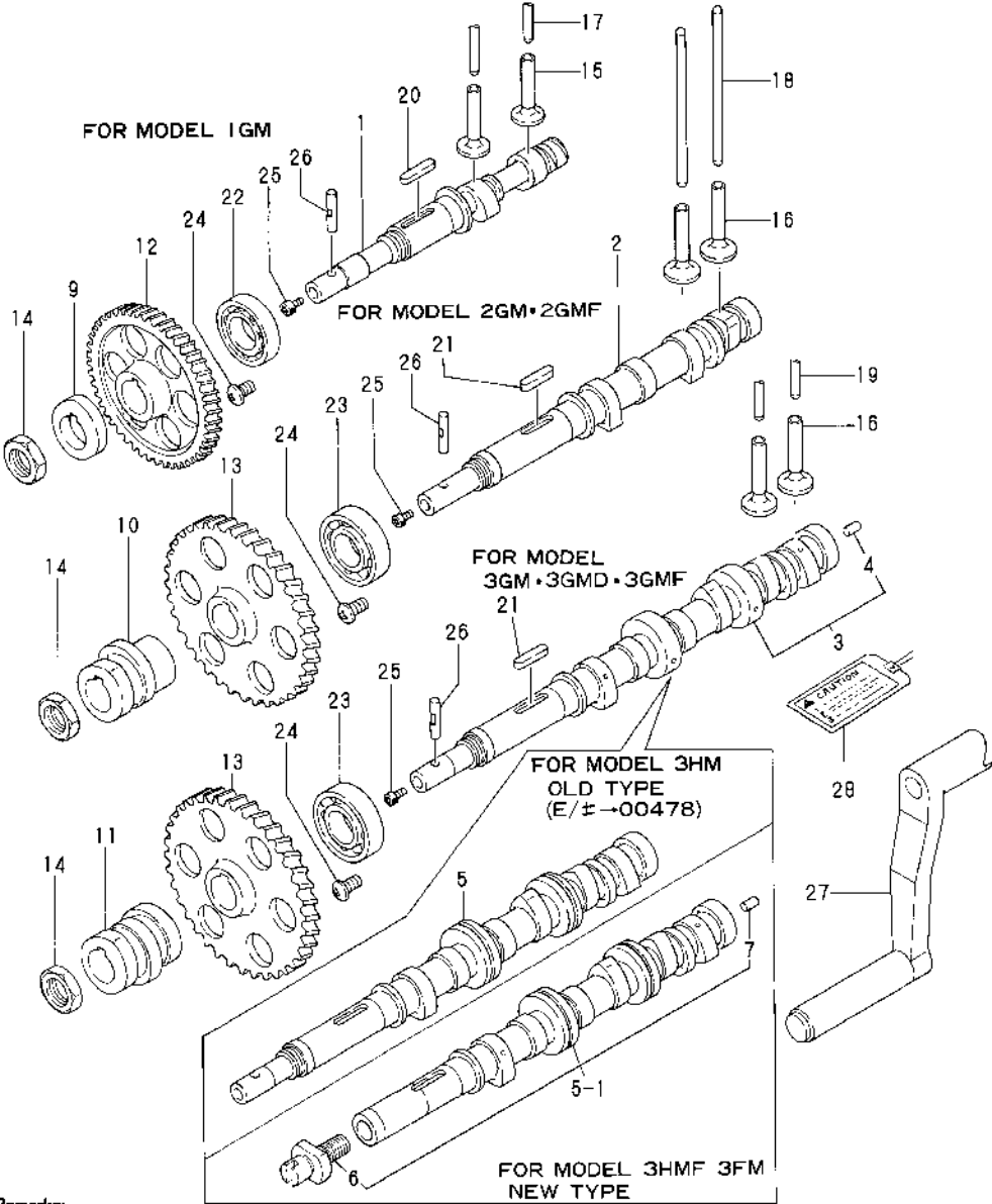
Fig.17. CAMSHAFT
