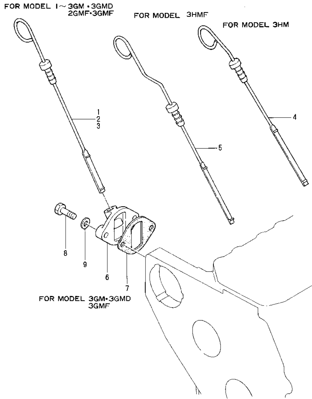
Fig.22. LUB. OIL DIPSTICK
