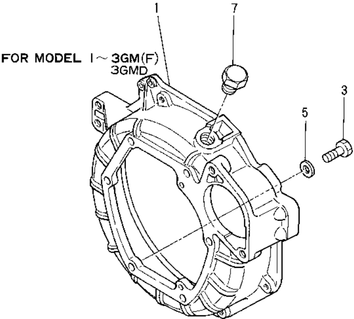
Fig.4. FLYWHEEL HOUSING
