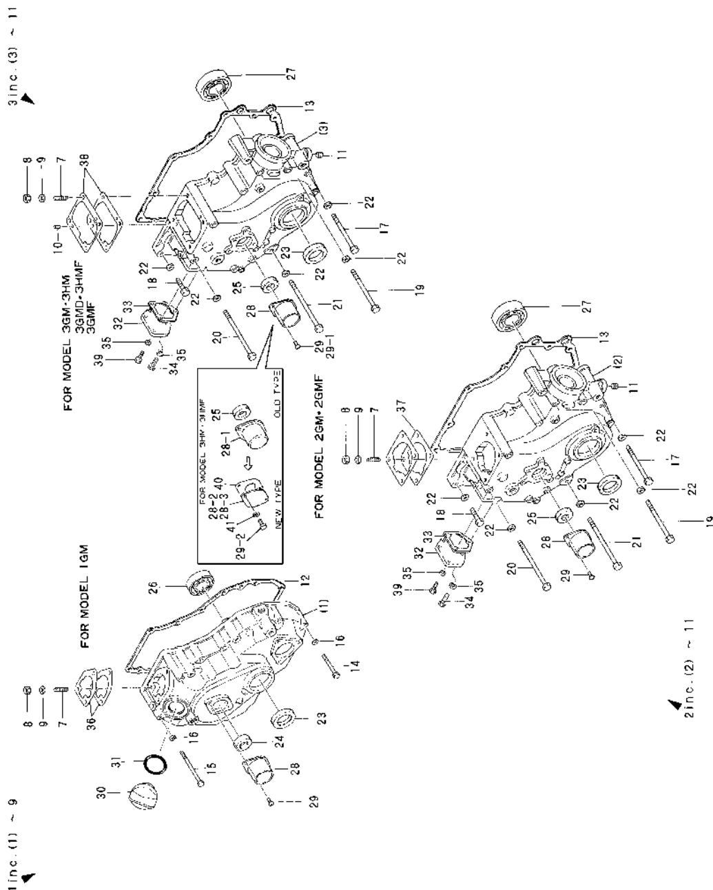
Fig.3. GEAR HOUSING
