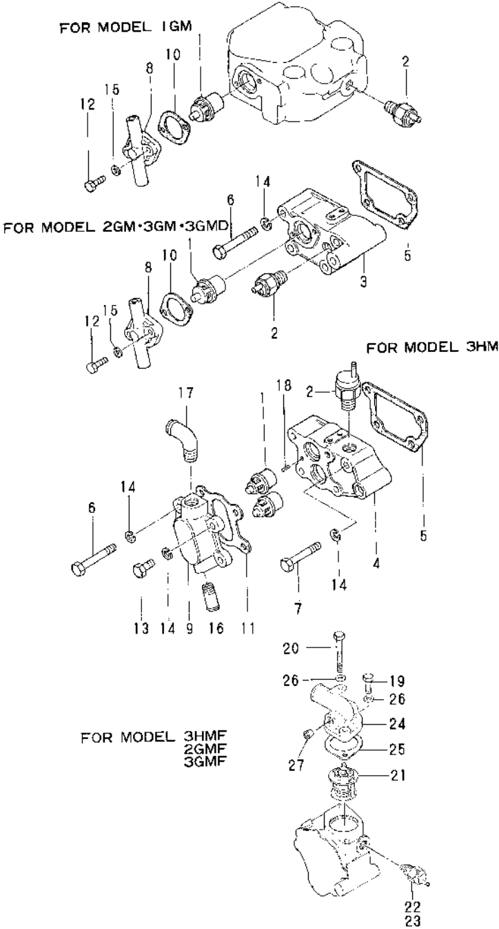
Fig.33. THERMOSTAT
