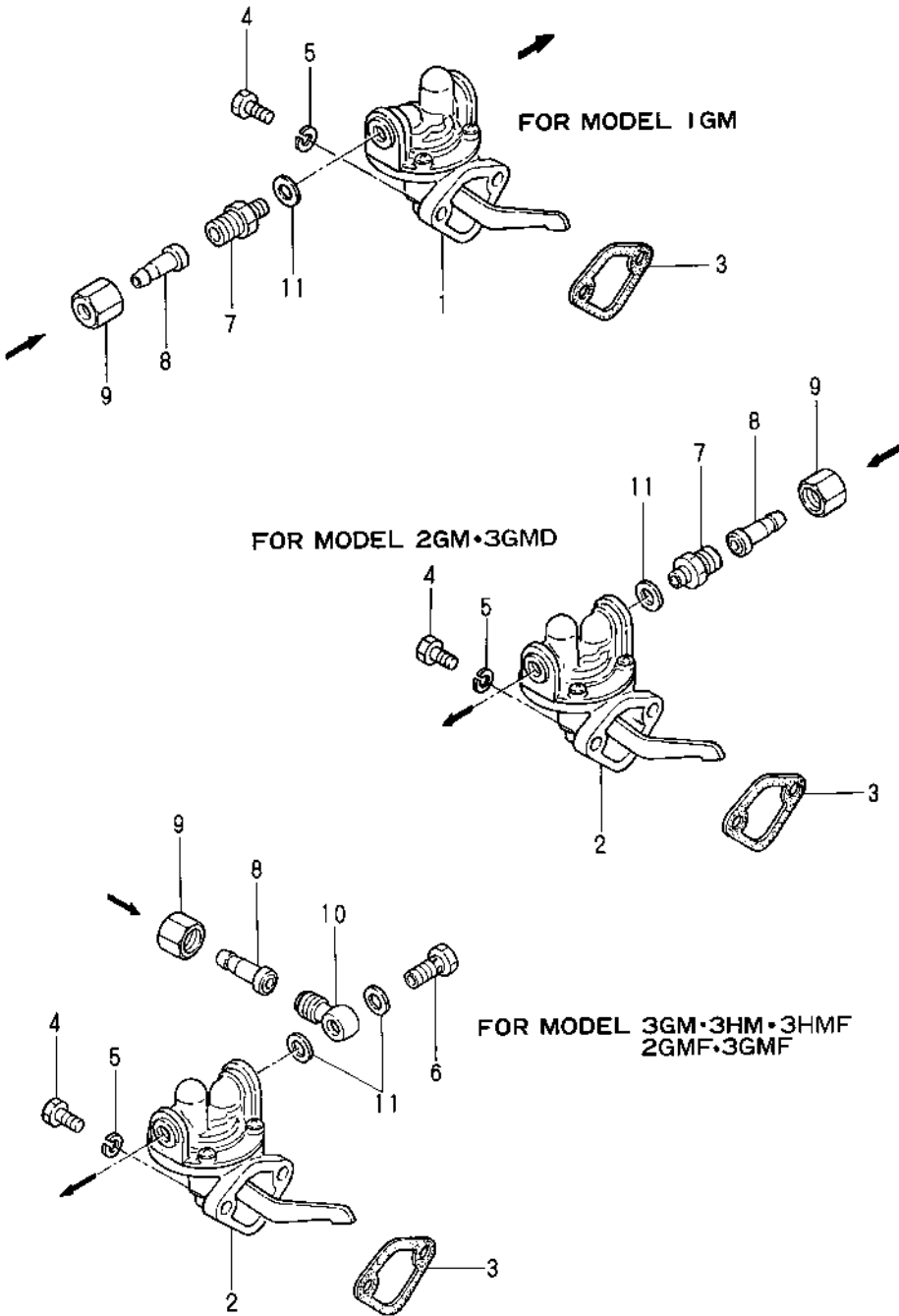
Fig.35. FUEL FEED PUMP
