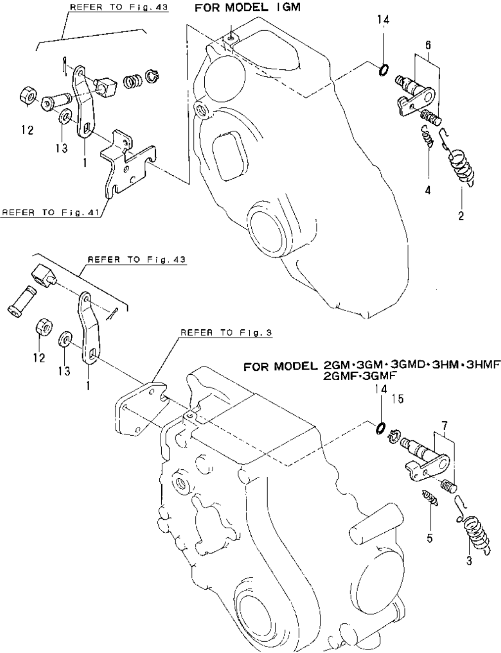
Fig.40. REGULATOR LINKS
