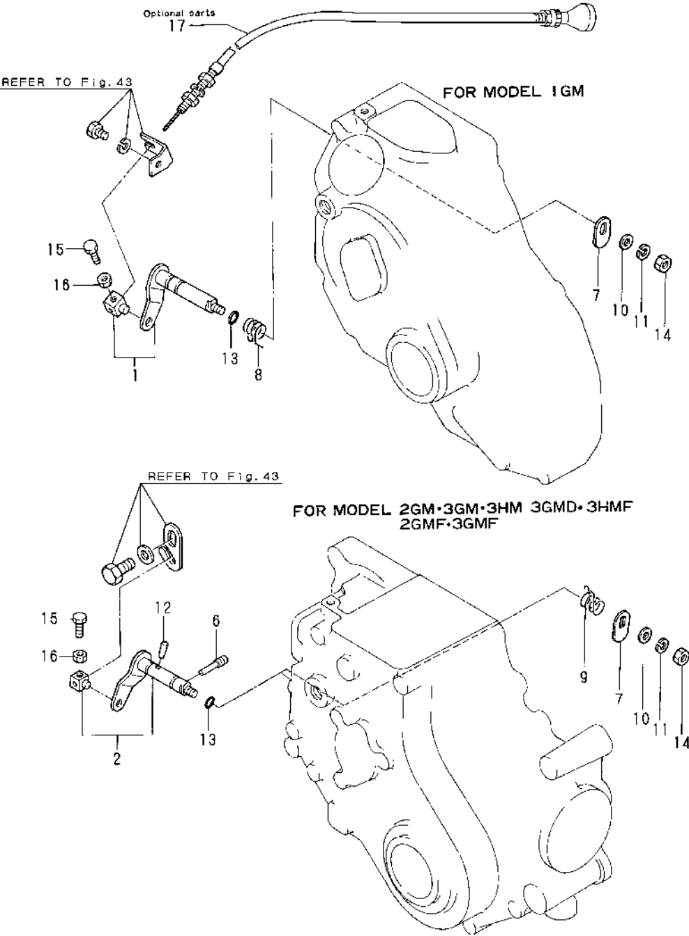
Fig.42. ENGINE STOP DEVIC
