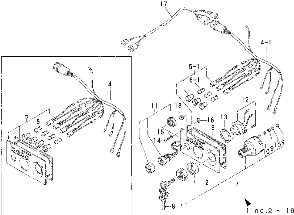
Fig.62. INSTRUMENT PANEL(S-TYPE/OPTIONAL)
