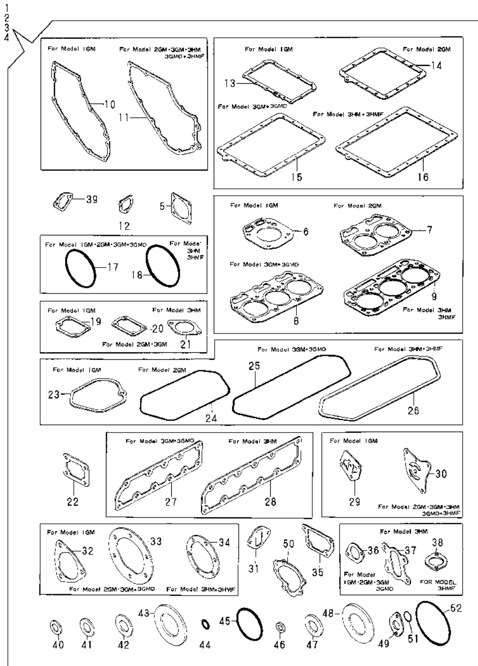
Fig.65. GASKET KIT(OPTIONAL)
