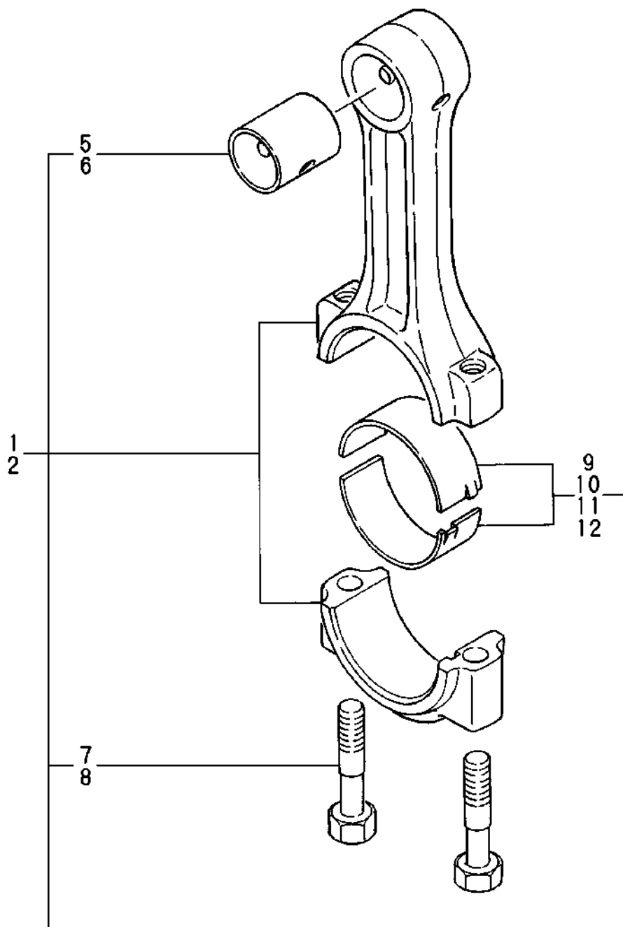
Fig.20. CONNECTING ROD
