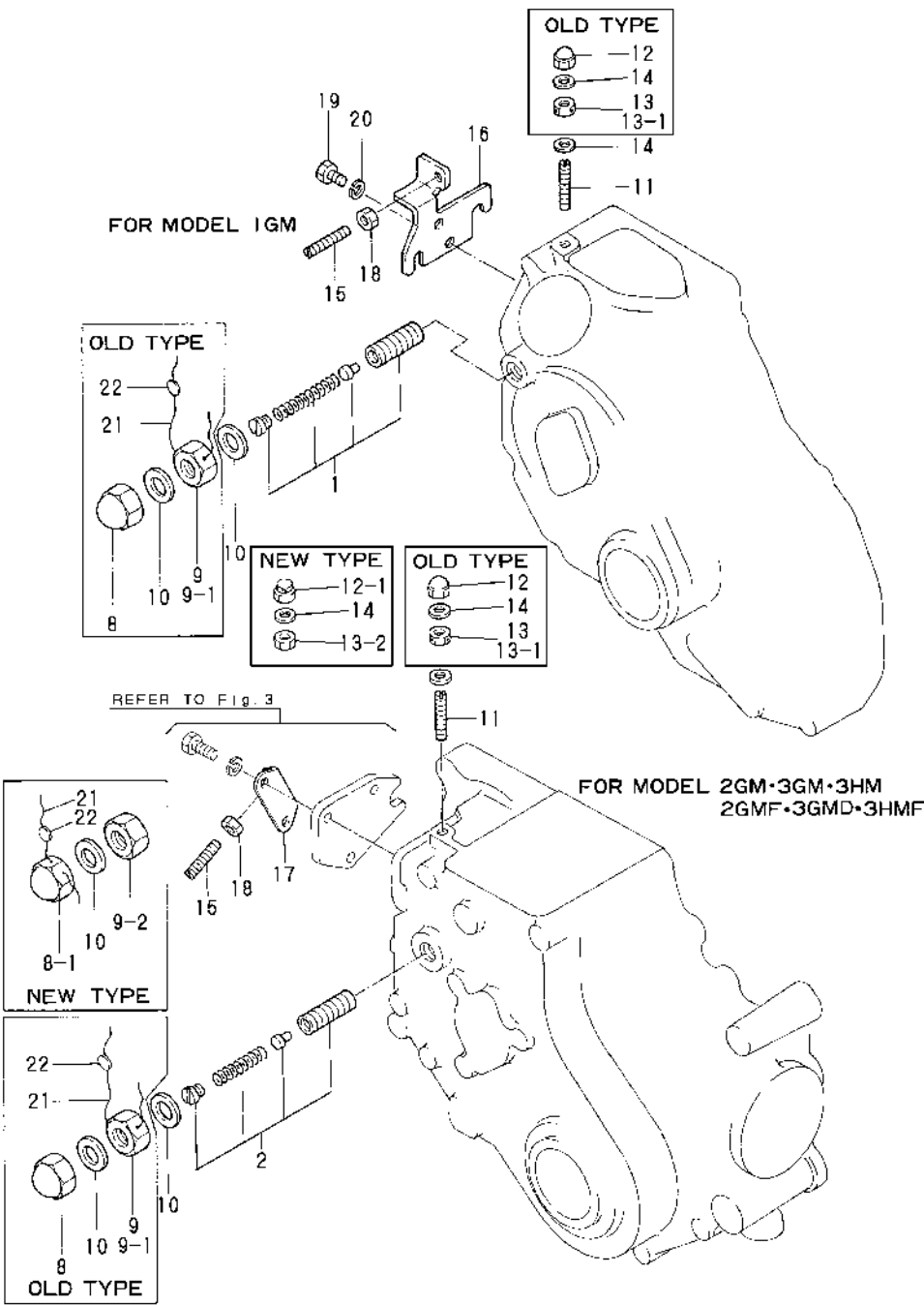
Fig.41. FUEL CONTROLLER
