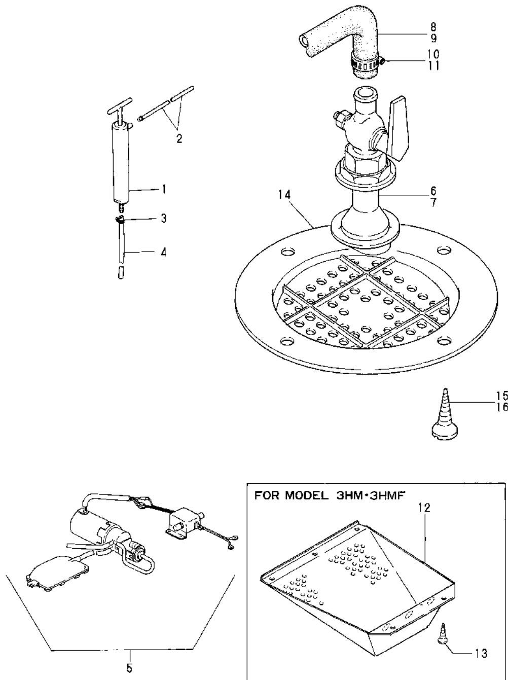
Fig.57. LUB. OIL WASTE,BILGE PUMP & KINGSTON COCK(OPTIONAL)
