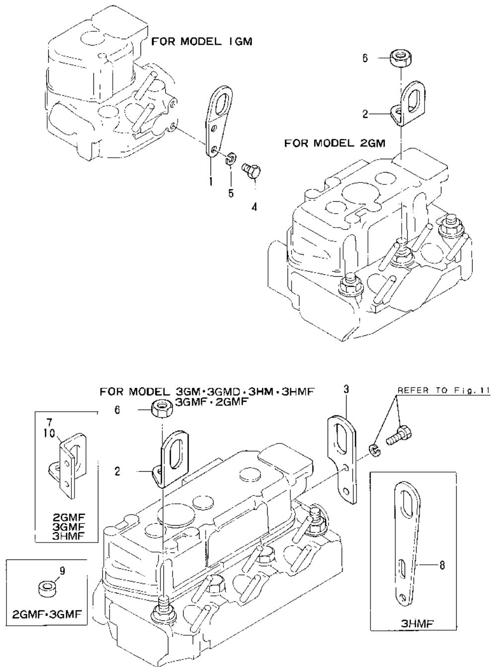
Fig.9. ENGINE LIFTER
