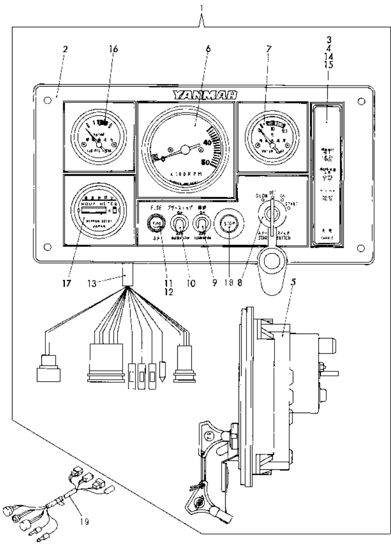
計器盤 (Cタイプ, 旧形) Fig. 41 INSTRUMENT PANEL (C-TYPE, PREVIOUS)
