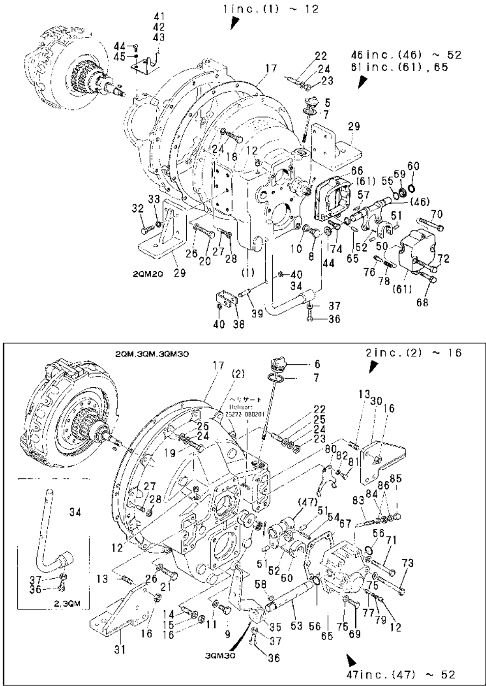
Fig.22. CLUTCH HOUSING
