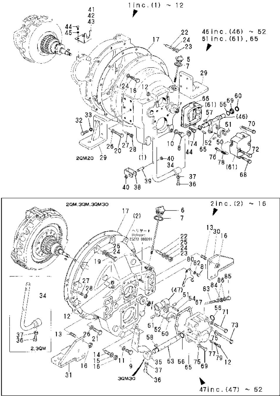
Fig.22. CLUTCH HOUSING
