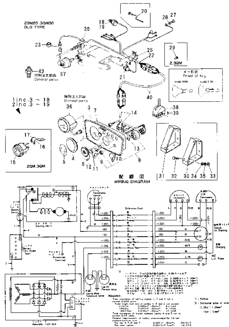
Fig.20. INSTRUMENT PANEL
