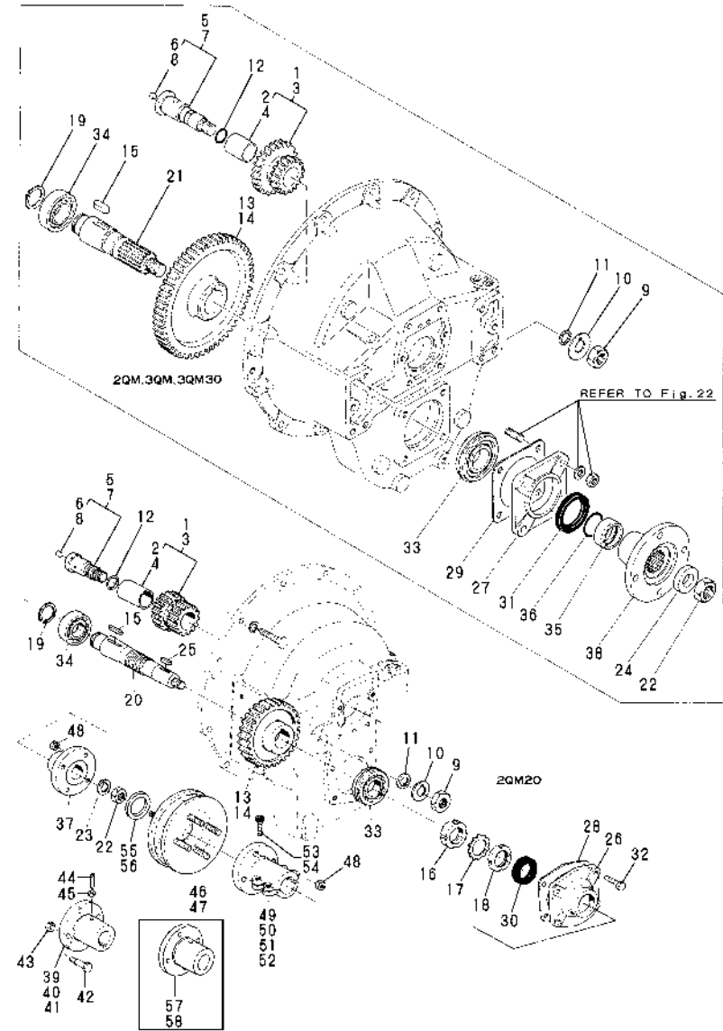
Fig.24. IDLE GEAR SHAFT & THRUST SHAFT
