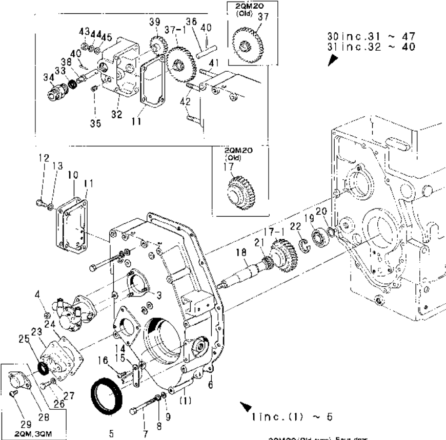
Fig.2. GEAR HOUSING
