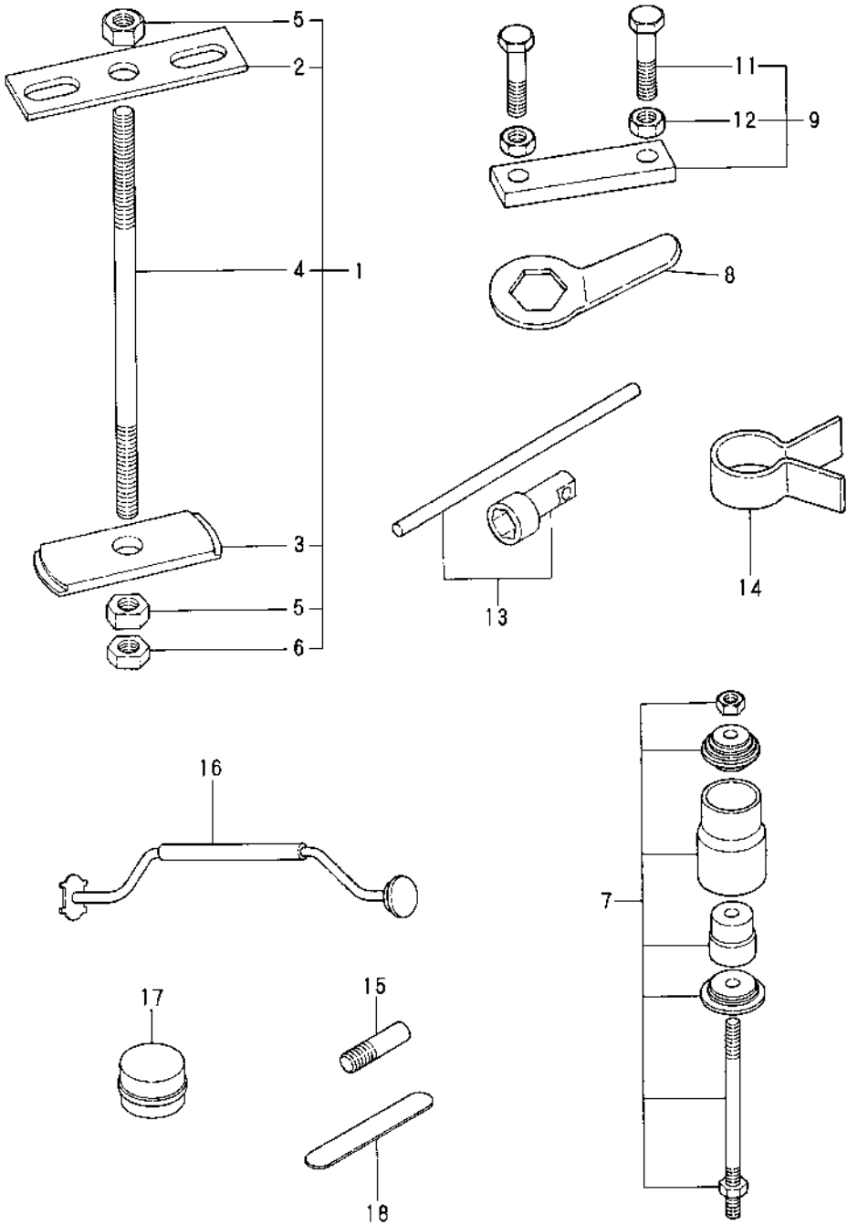
Fig.26. SPECIAL TOOL(OPTIONAL)
