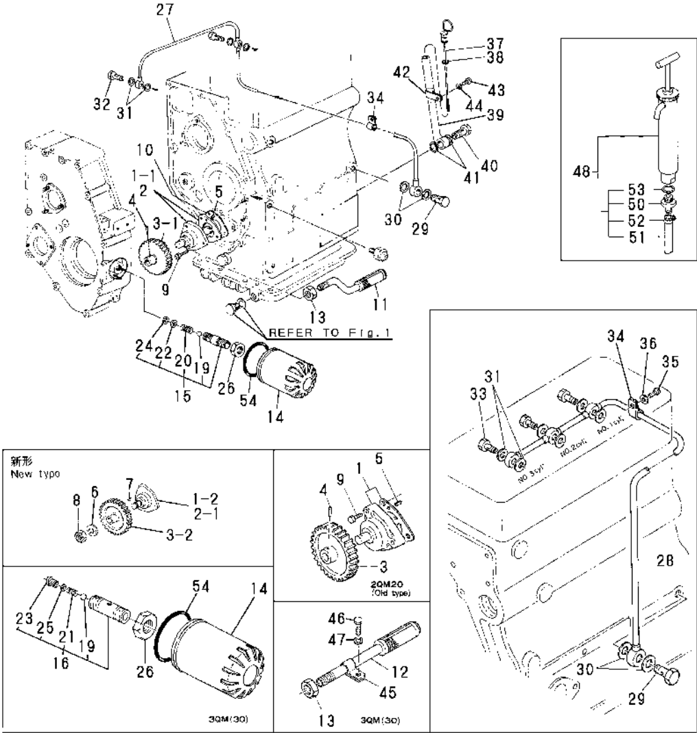
Fig.8. LUB.OIL SYSTEM
