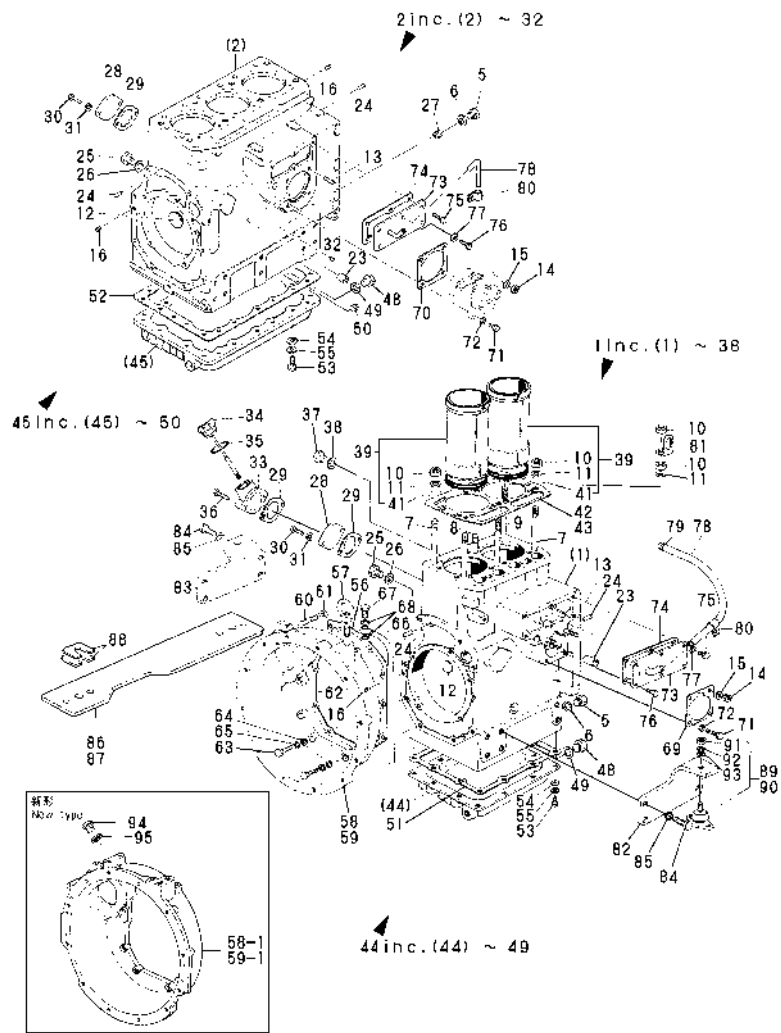
Fig.1. CYLINDER BLOCK
