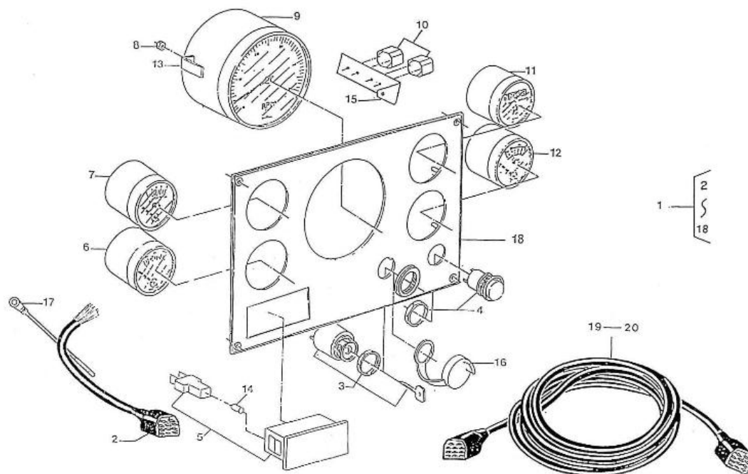
PANEL "C" (Optional equipment)
