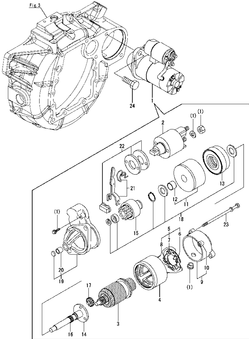
Fig.36. STARTER MOTOR
