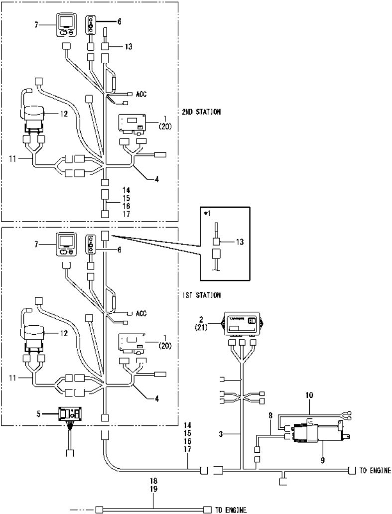
Fig.67. (49C)VC10(SINGLE ENGINE)(OPTIONAL)
