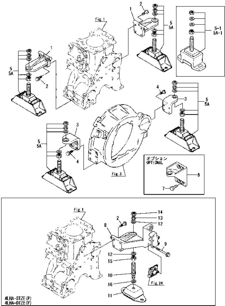
Fig.4. MOUNTING FOOT(4LHA-ST/DT(Z)E(P))
