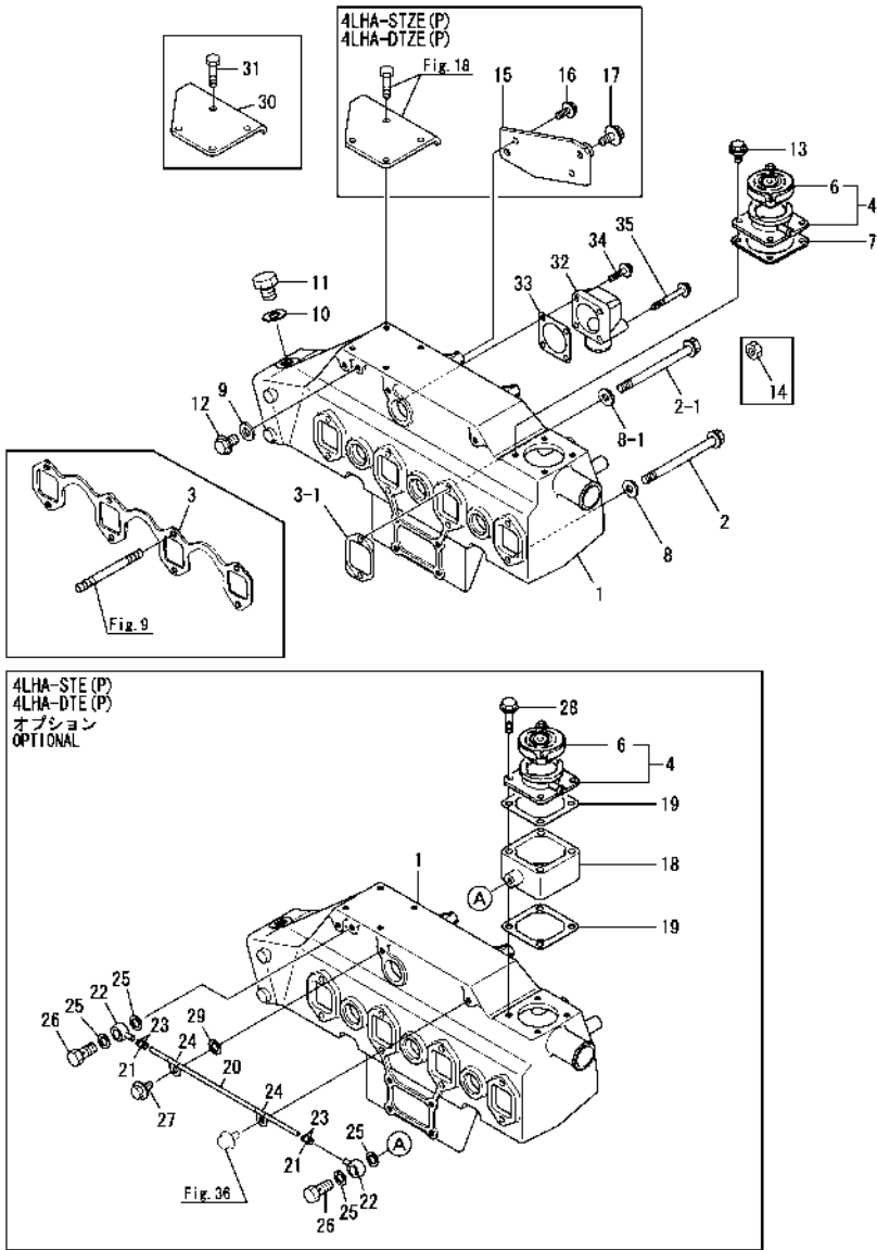
Fig.13. EXHAUST MANIFOLD
