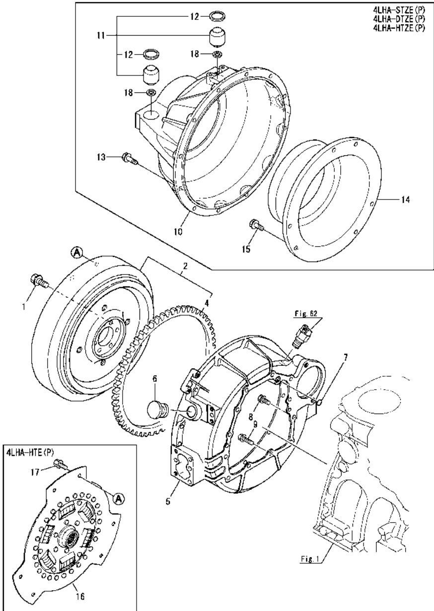
Fig.3. FLYWHEEL HOUSING
