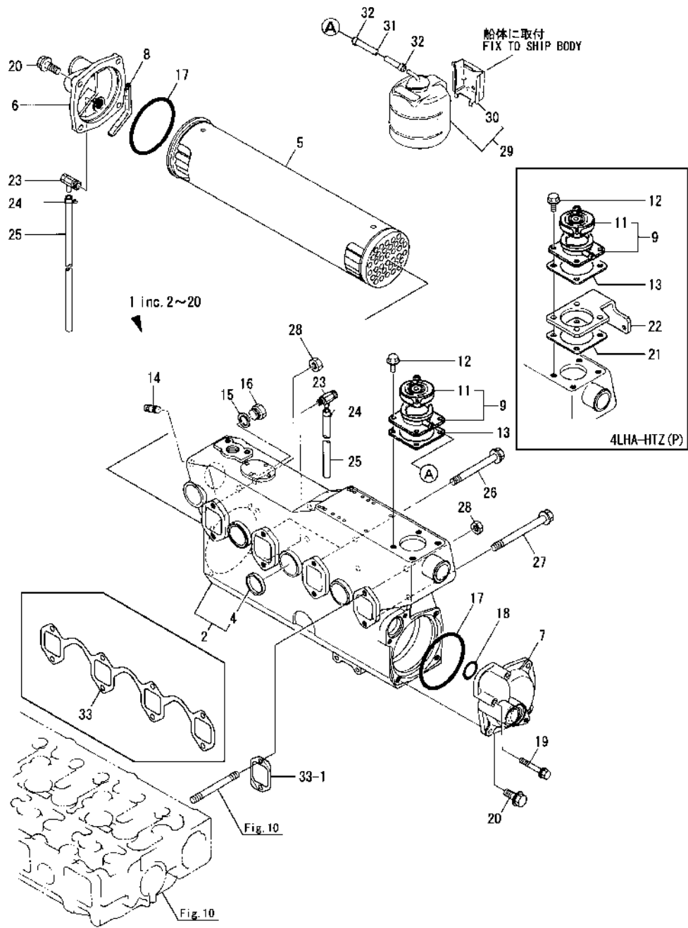
Fig.32. C.F.W.COOLER(4LHA-HT(Z)E(P))
