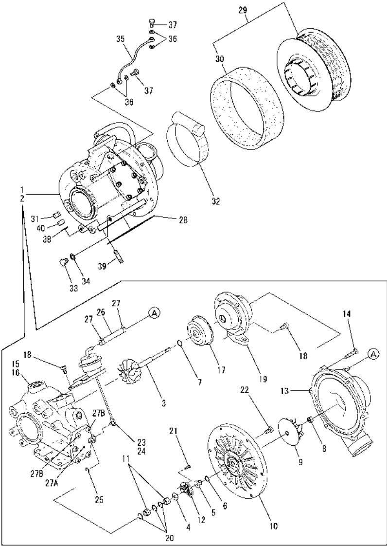
Fig.9. TURBINE
