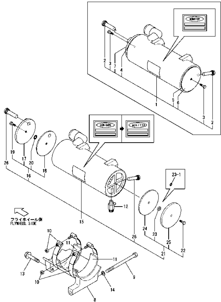
Fig.25. LUB. OIL COOLER(6LP-ST(Z)E(P)1)
