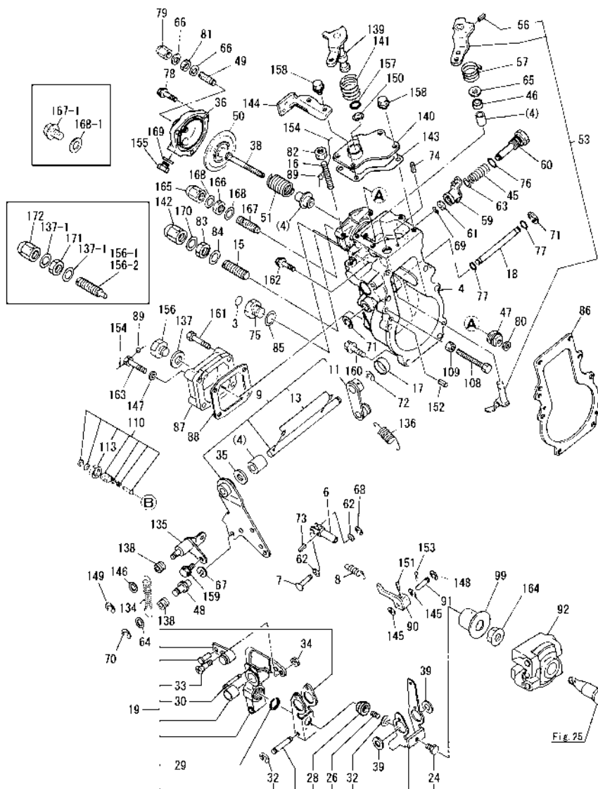
Fig.28. GOVERNOR
