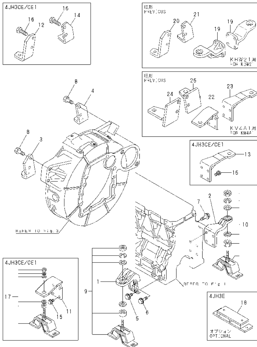
Fig.6. MOUNTING FOOT(4JH3E)
