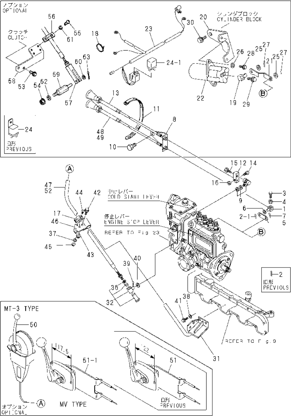
OCR10-M46701 4JH3E(CE/CE1)-TE(TCE) Fig.44. ENGINE STOP DEVIC(4JH3E)
