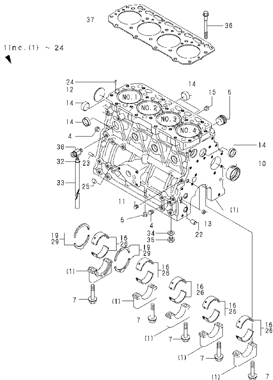
Fig.1. CYLINDER BLOCK(4JH3E)
