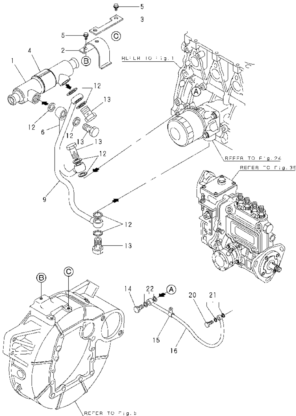
Fig.21. LUB.OIL COOLER(4JH3E)
