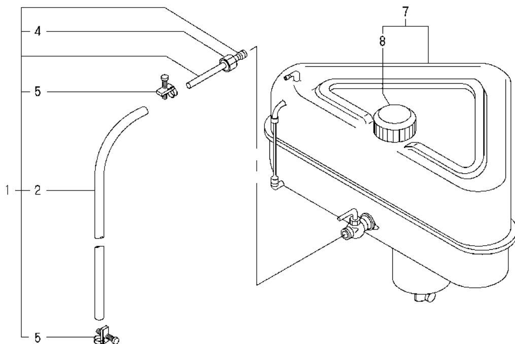
Fig.43. FUEL TANK
