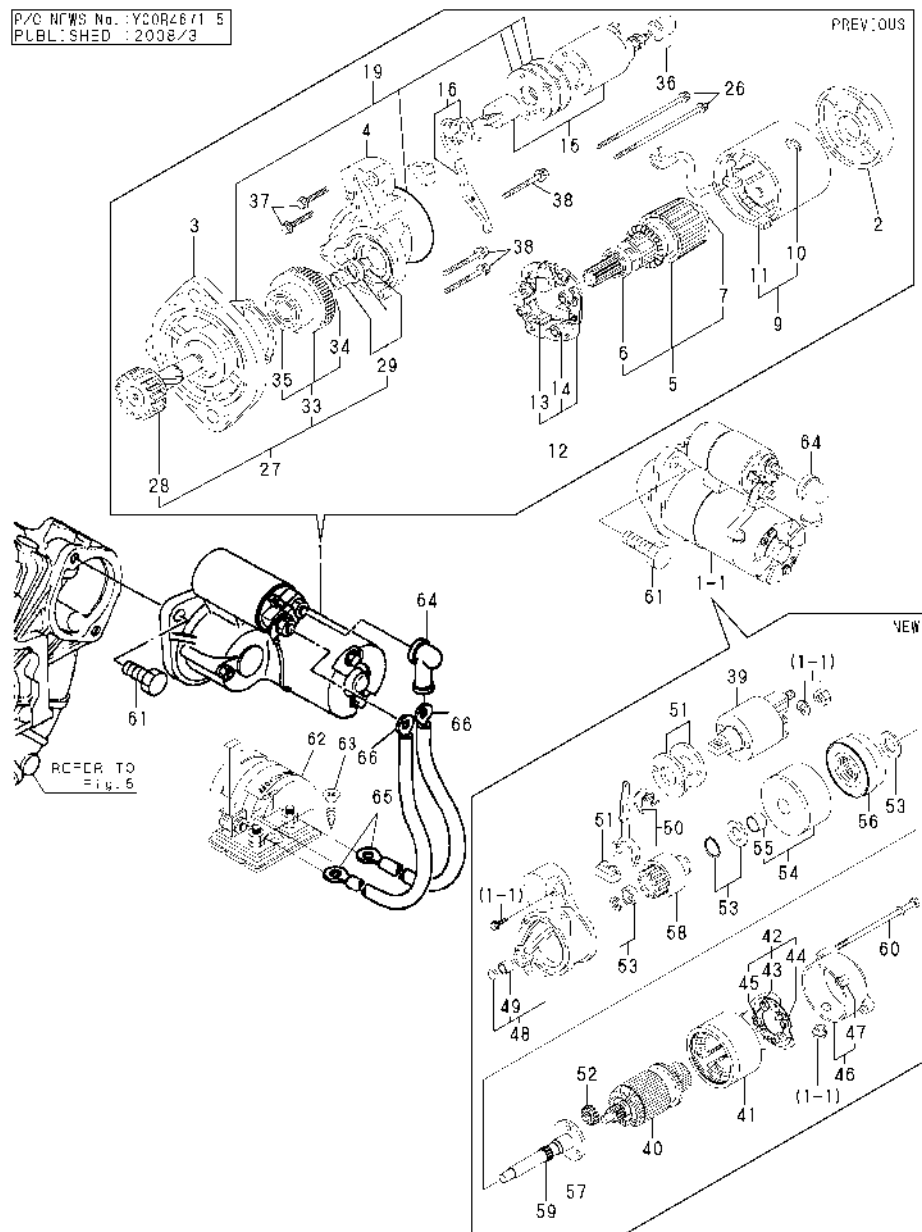
Fig.47. STARTING MOTOR(4JH3-TE)
