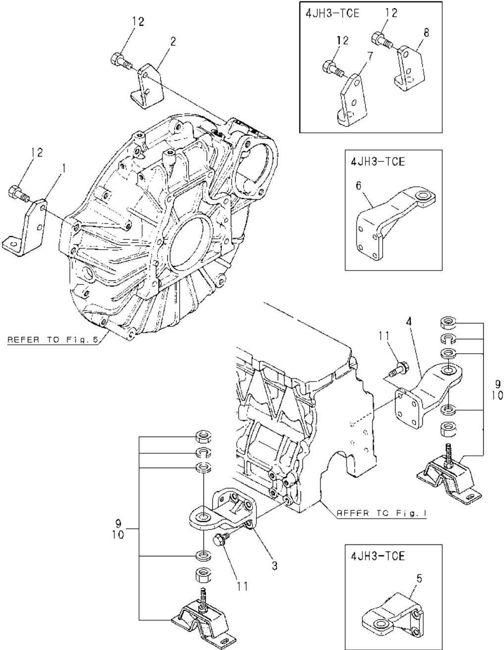
0CR10-M46701 4JH3E(CE/CE1)-TE(TCE) Fig.7. MOUNTING FOOT(4JH3-TE)
