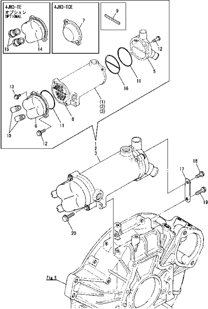
Fig.22. LUB.OIL COOLER(4JH3-TE)
