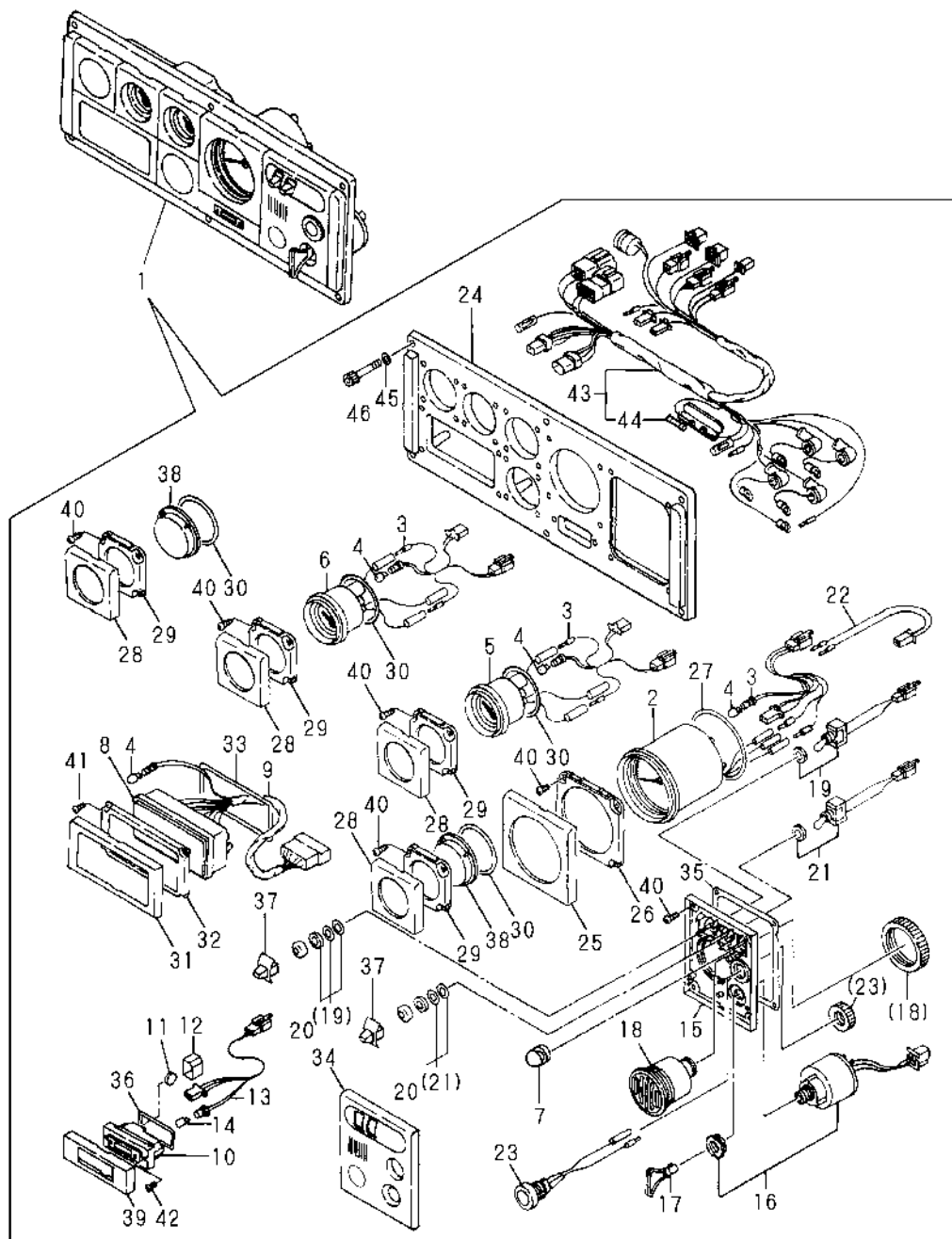
Fig.69. PANEL(D:NEW TYPE:4JH3-TE)
