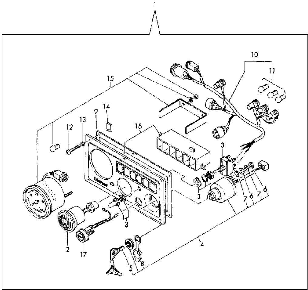
Fig.57. INSTRUMENT PANEL(B:4JH3-TE)
