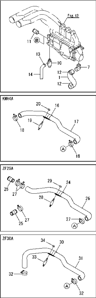
Fig.23. COOLING SEA WATER PIPE(4JH4-HT/HT1)
