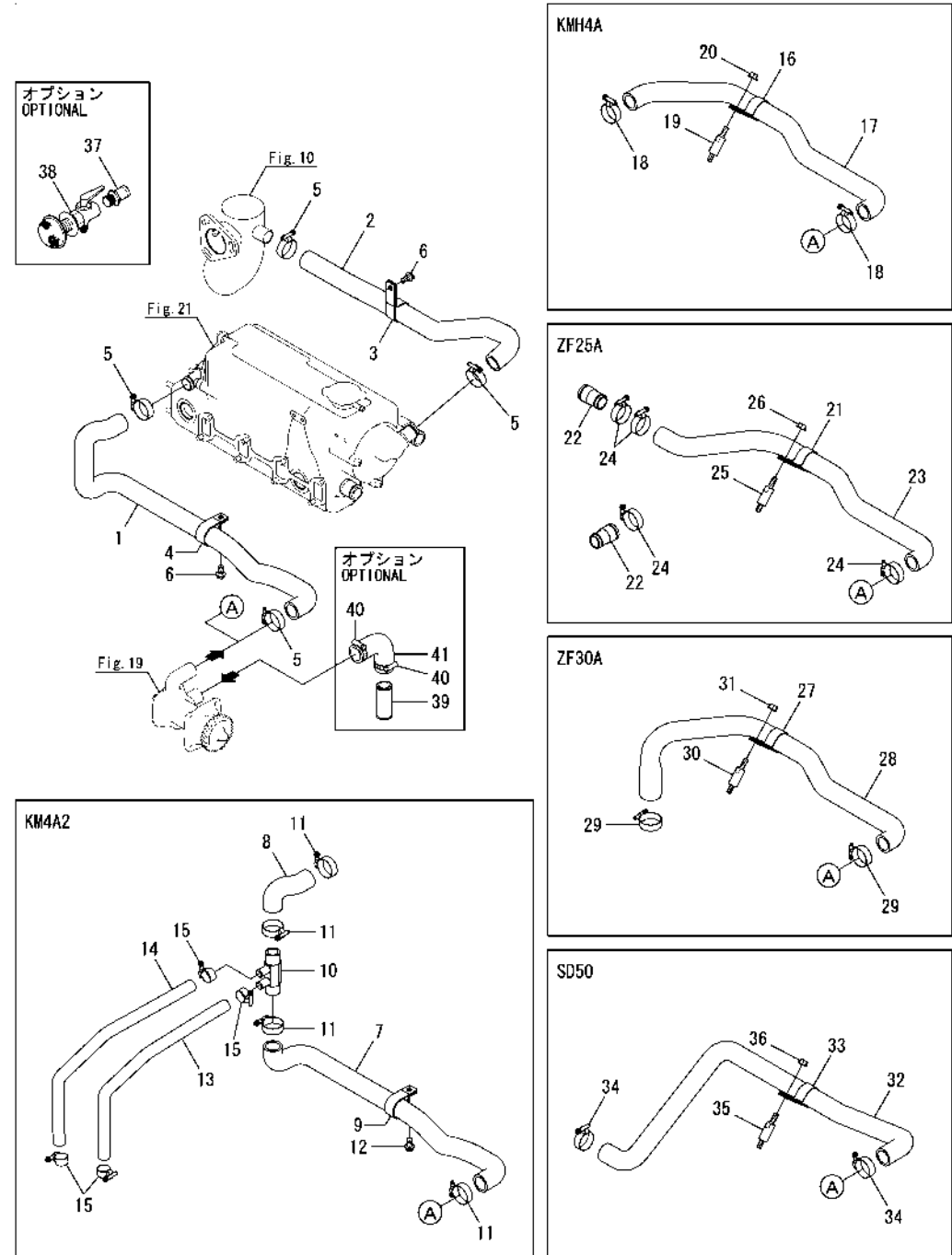
Fig.22. COOLING SEA WATER PIPE(4JH4-TE)
