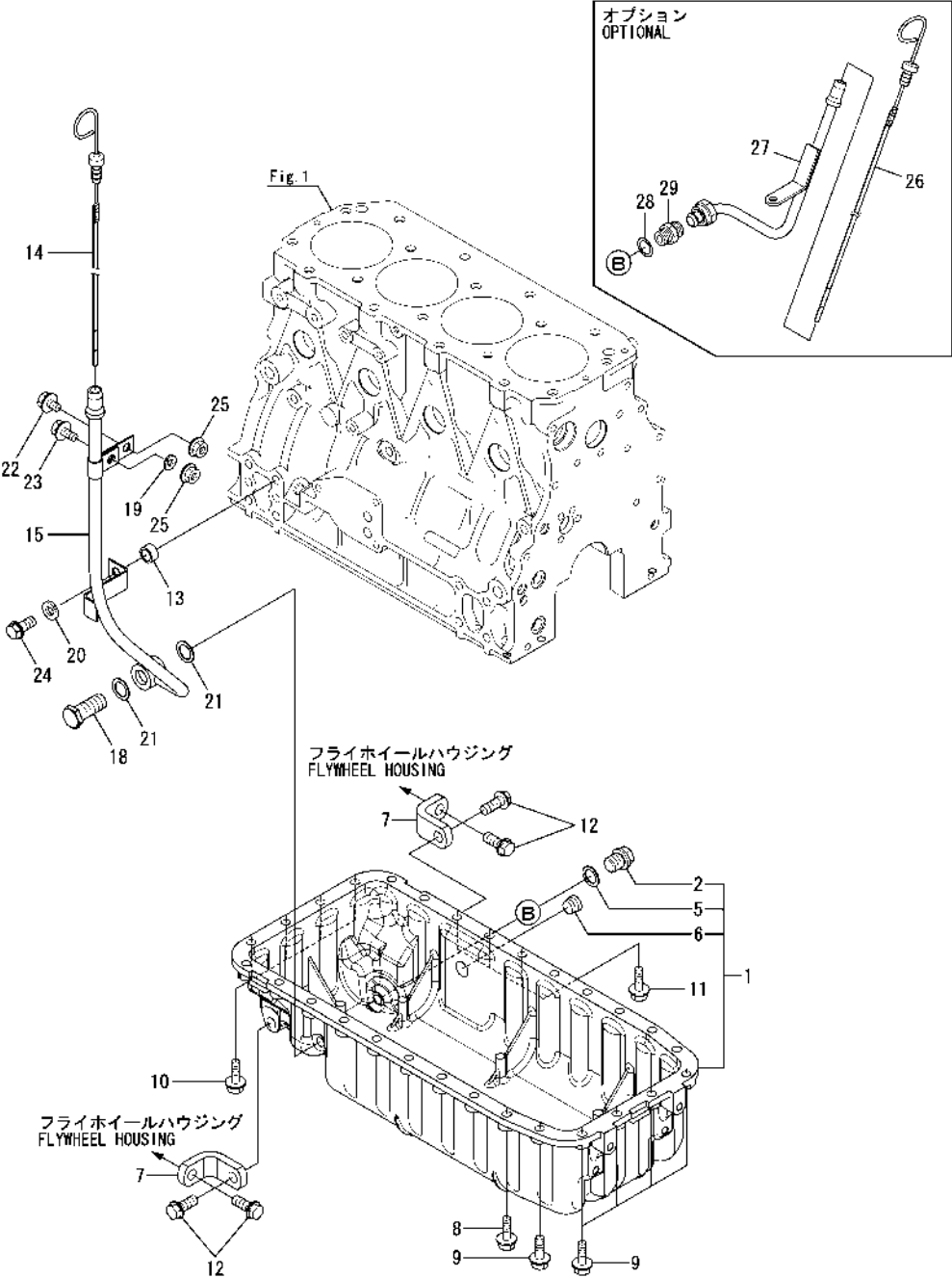
Fig.5. LUB.OIL SUMP
