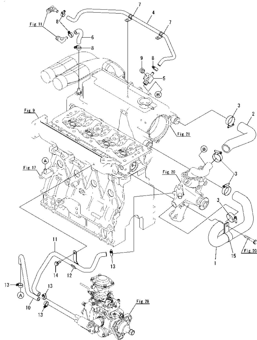
Fig.24. COOLING FRESH WATER PIPE
