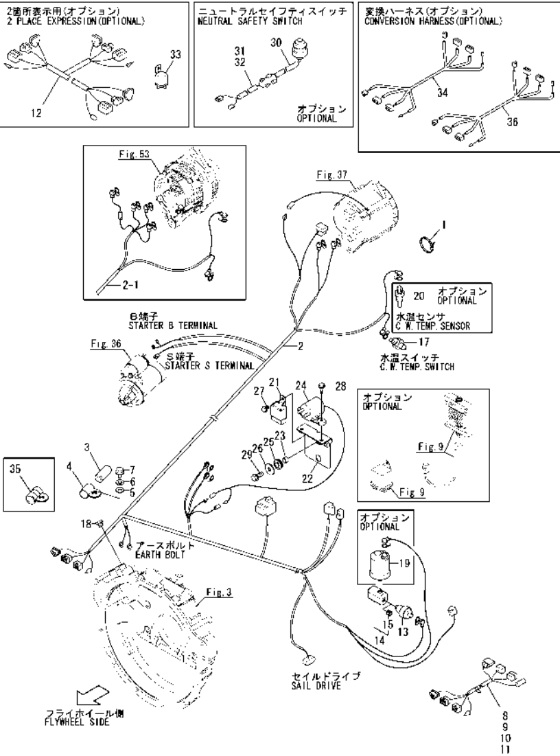
Fig.42. WIRE HARNESS & SENSOR
