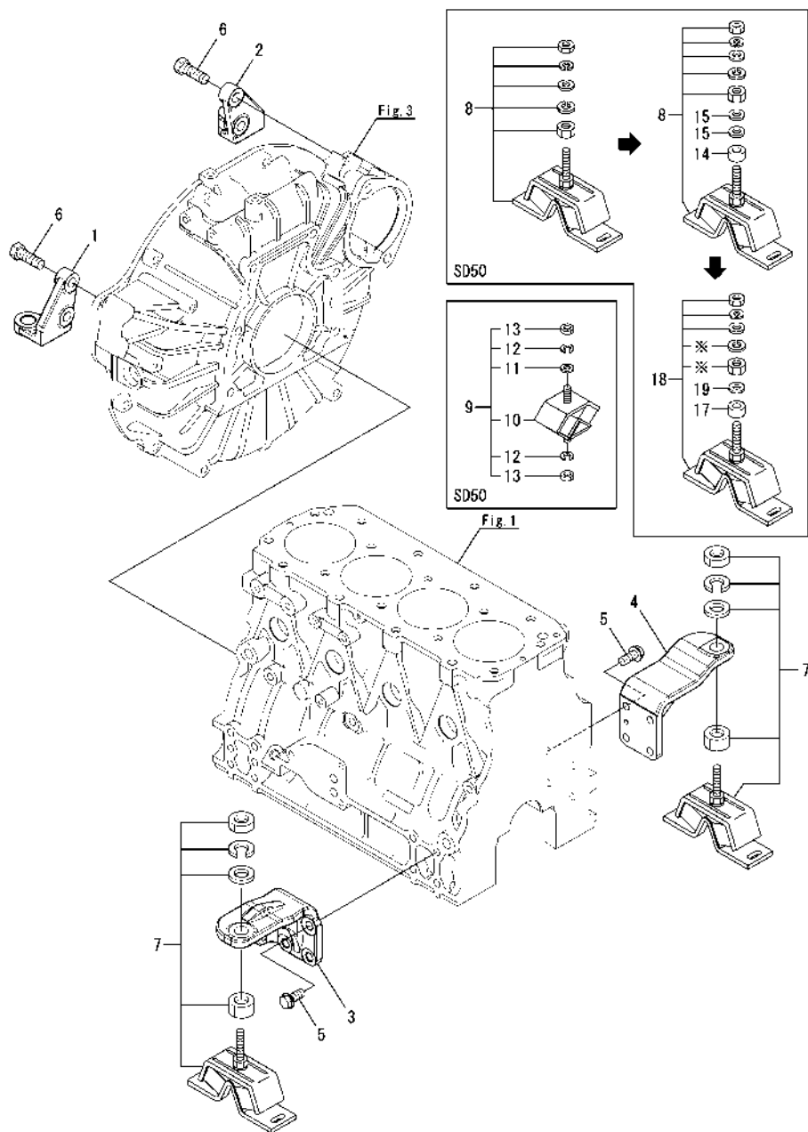
Fig.4. MOUNTING FOOT
