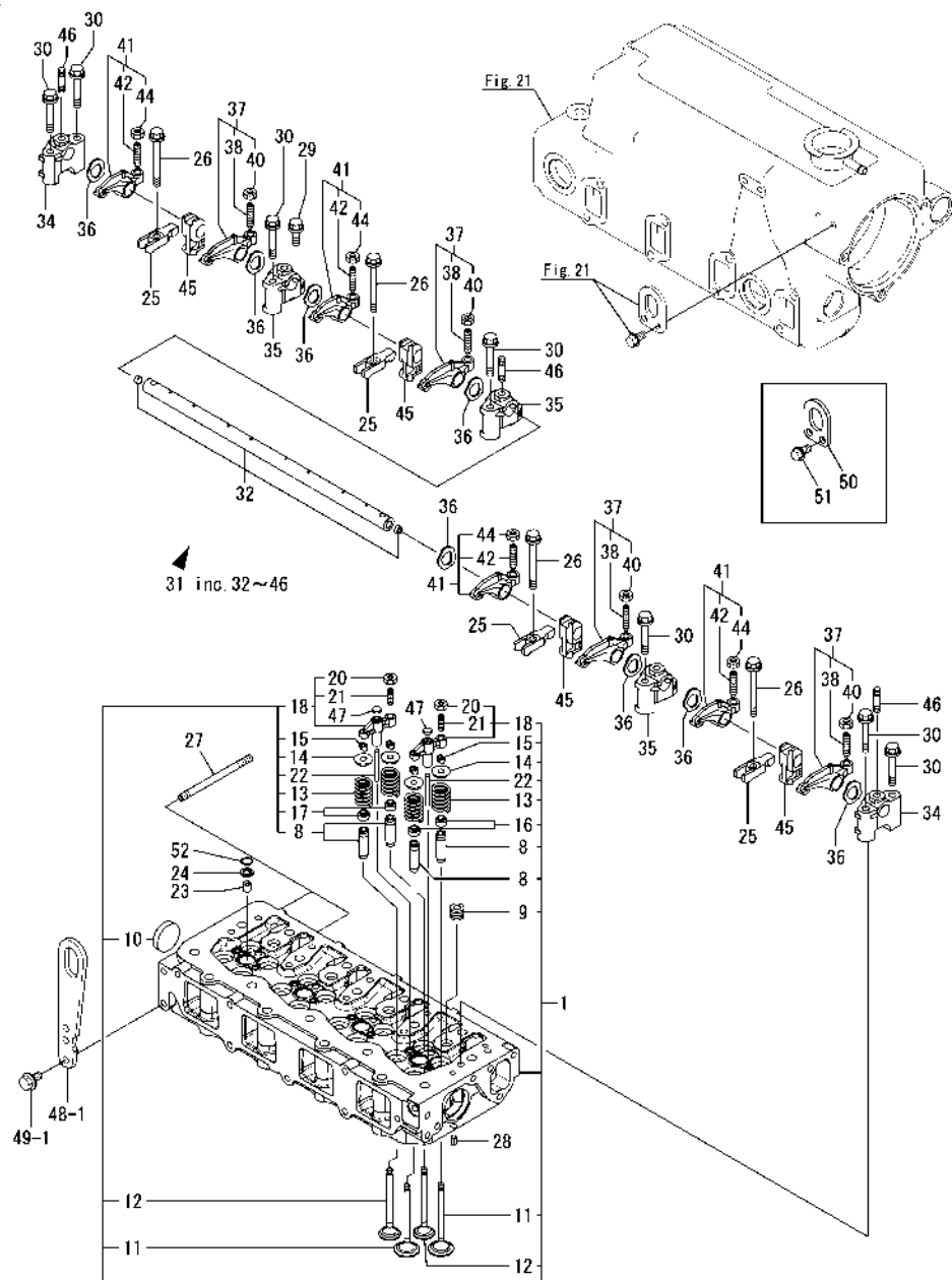
Fig.7. CYLINDER HEAD
