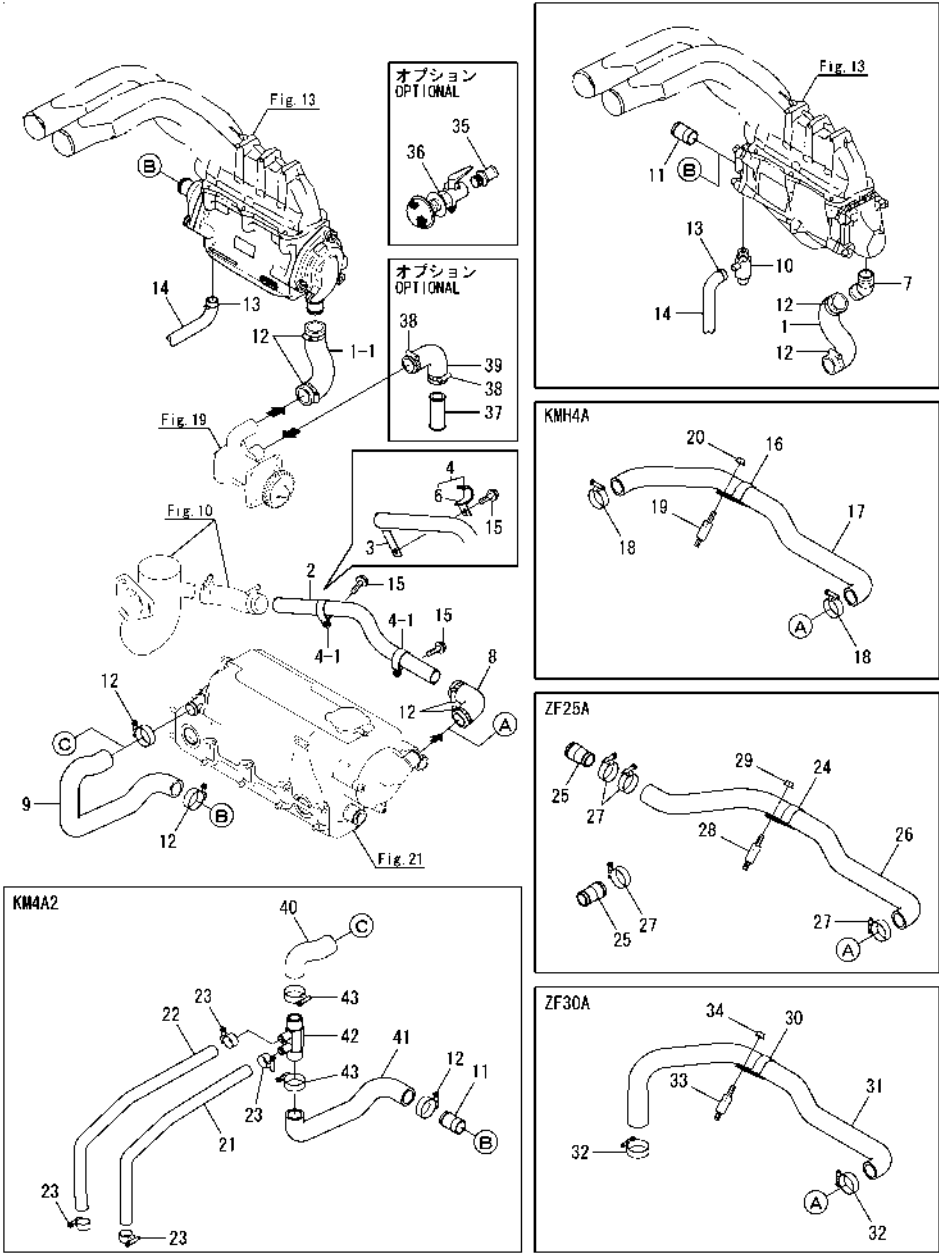
Fig.23. COOLING SEA WATER PIPE(4JH4-HT/HT1)
