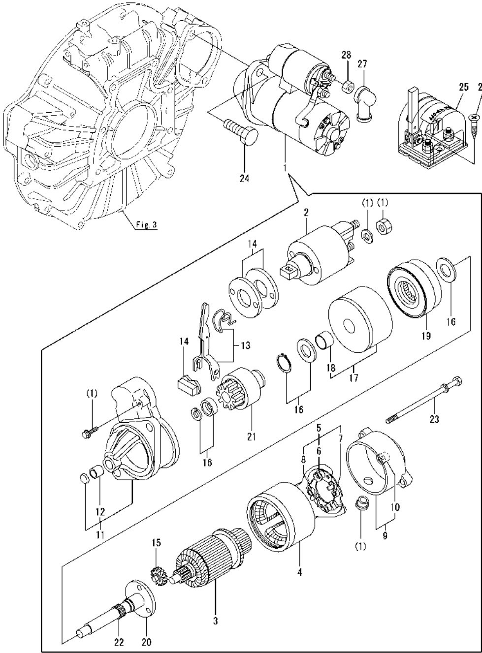
Fig.36. STARTING MOTOR
