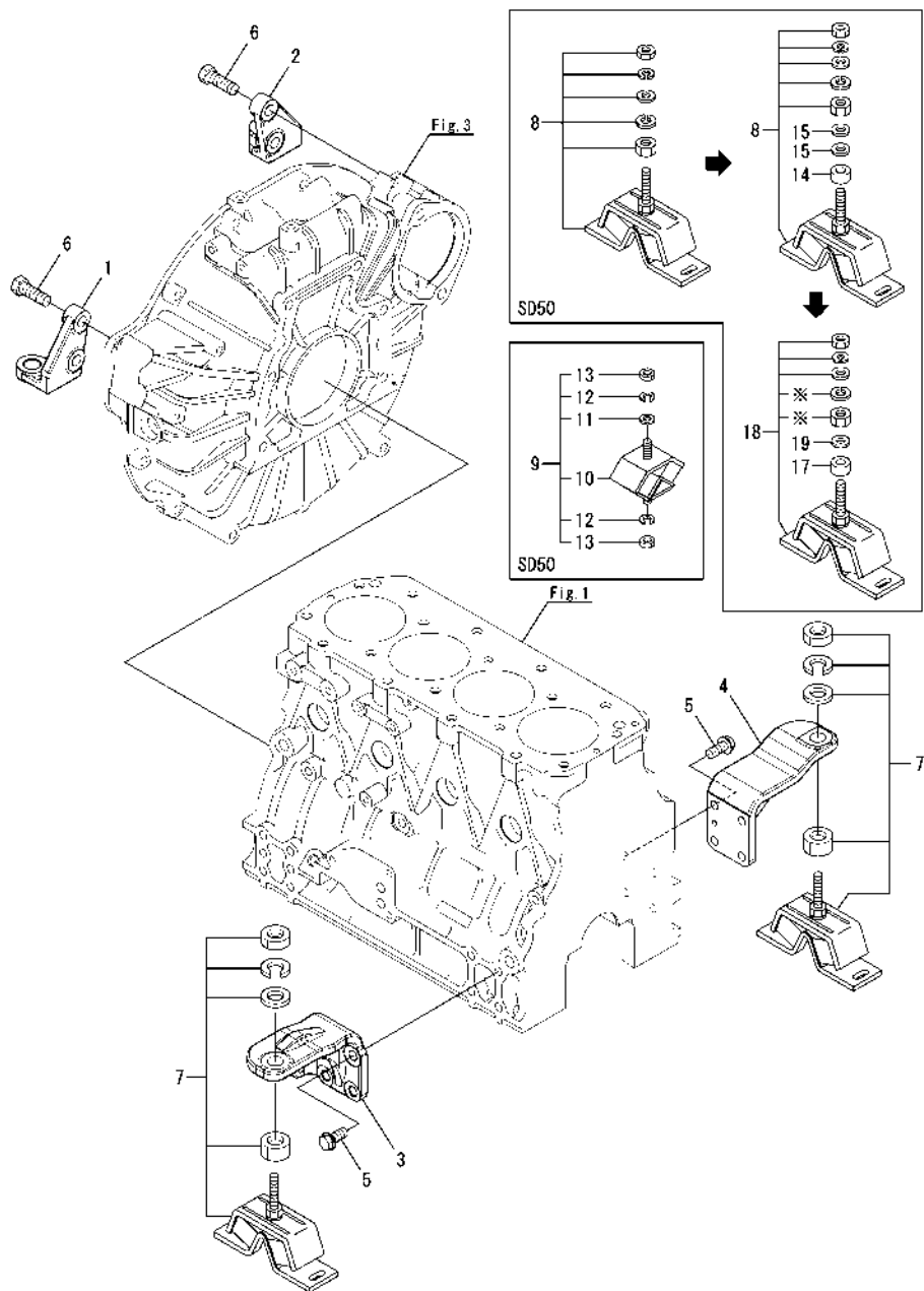
Fig.4. MOUNTING FOOT
