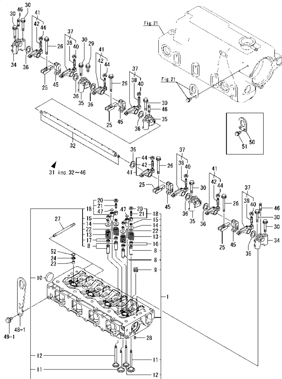
Fig.7. CYLINDER HEAD
