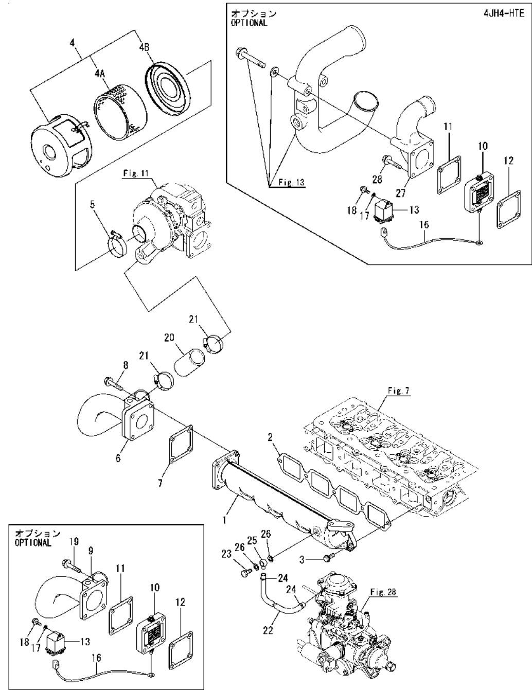
Fig.9. SUCTION MANIFOLD
